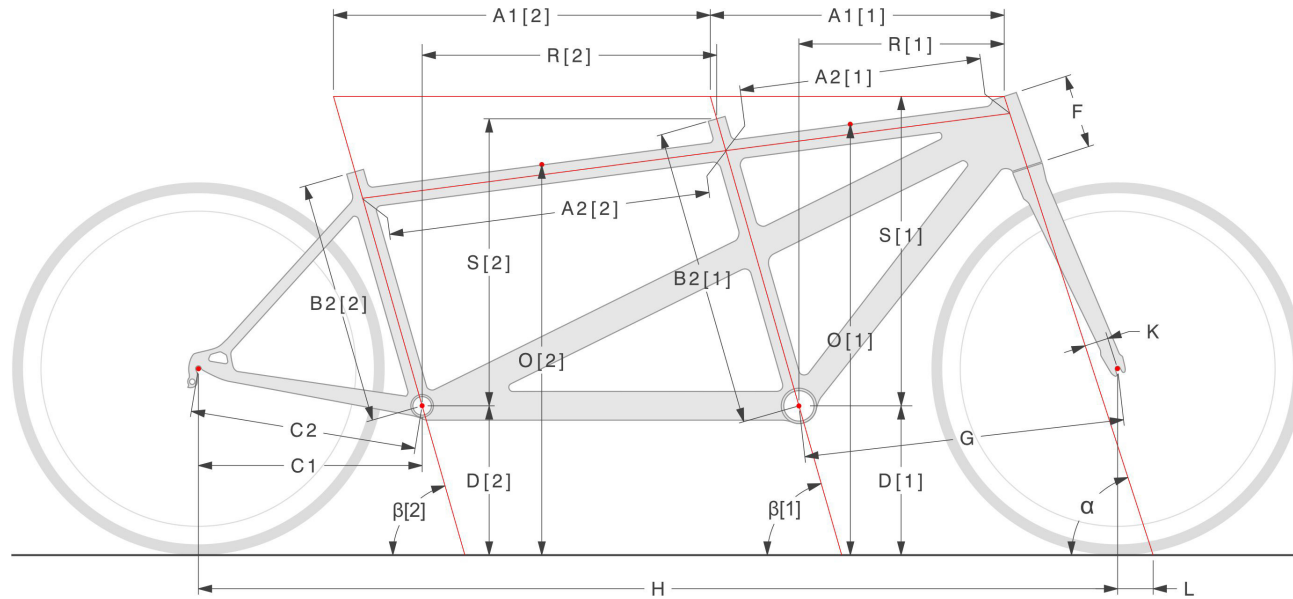
Wheels 25-622 (700x25C)
